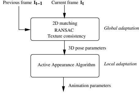
Fig. 4.5. Summary of the feature/appearance-based tracker.
