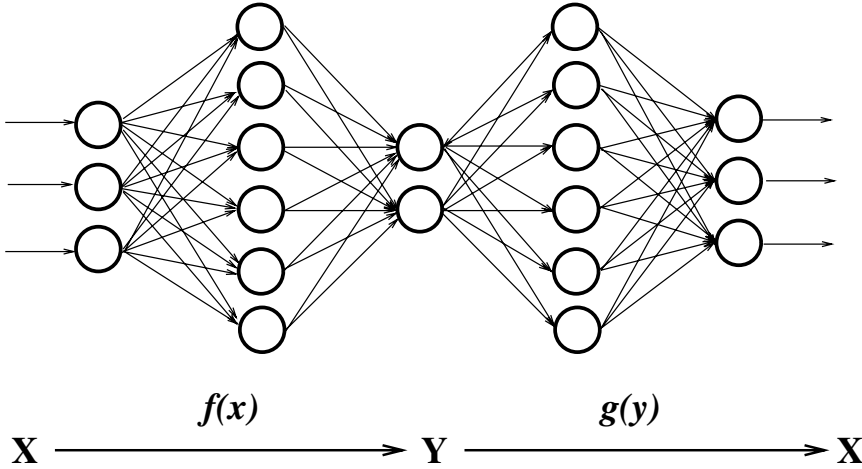
Fig. 7.9. Autoassociative (“bottleneck”) neural network for computing principal manifolds \mathbf{y} \in \mathbb{R}^k in the input space \mathbf{x} \in \mathbb{R}^N .
